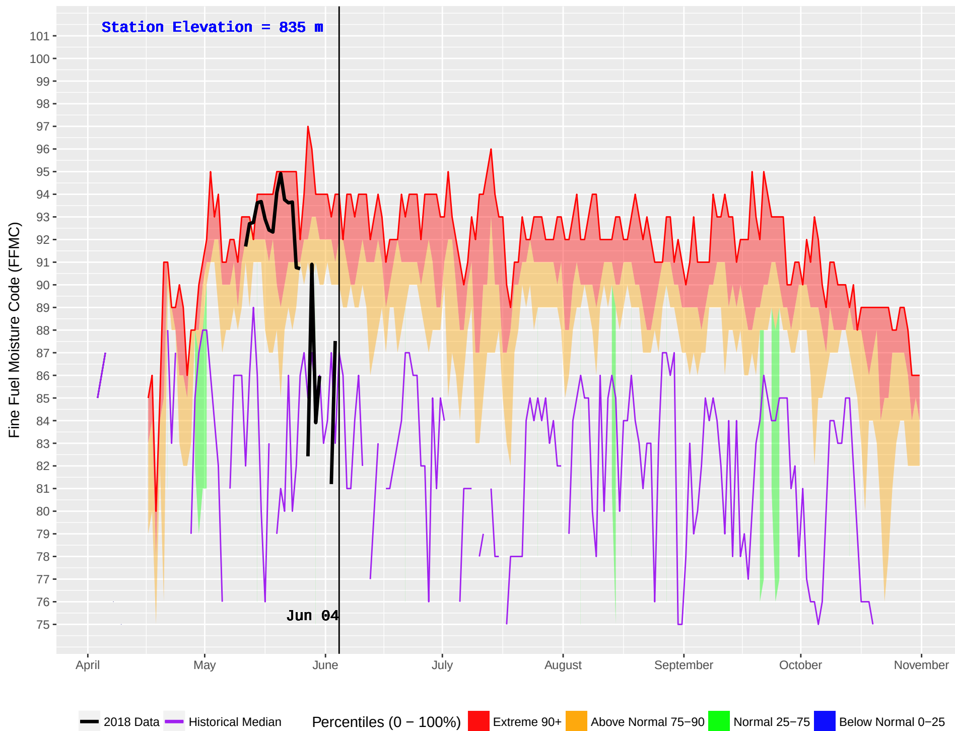
SILVER (120) : Historical (1986–2016) and Current (2018) Noon Fine Fuel Moisture Code (FFMC)
