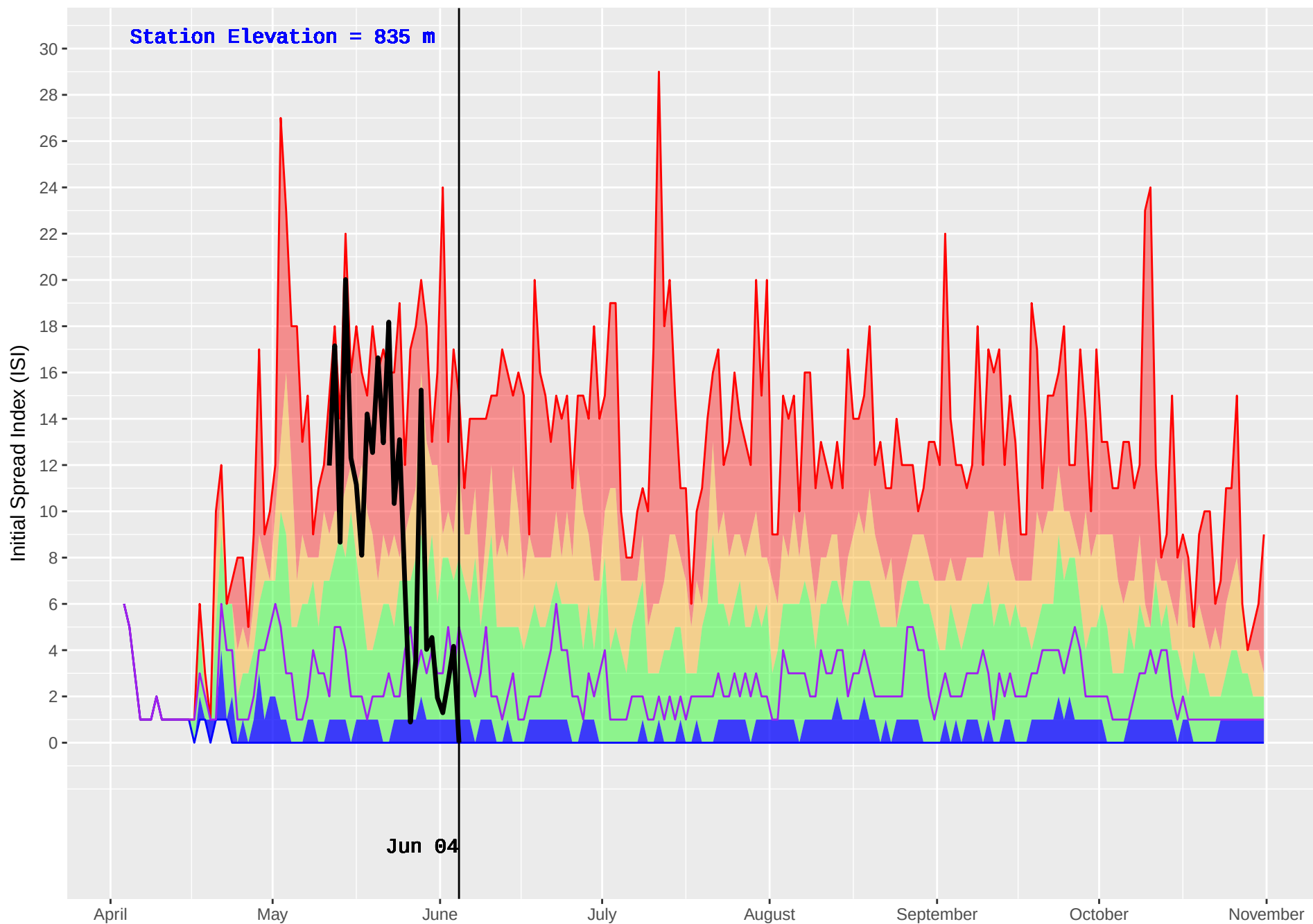
SILVER (120) : Historical (1986–2016) and Current (2018) Noon Initial Spread Index (ISI)
