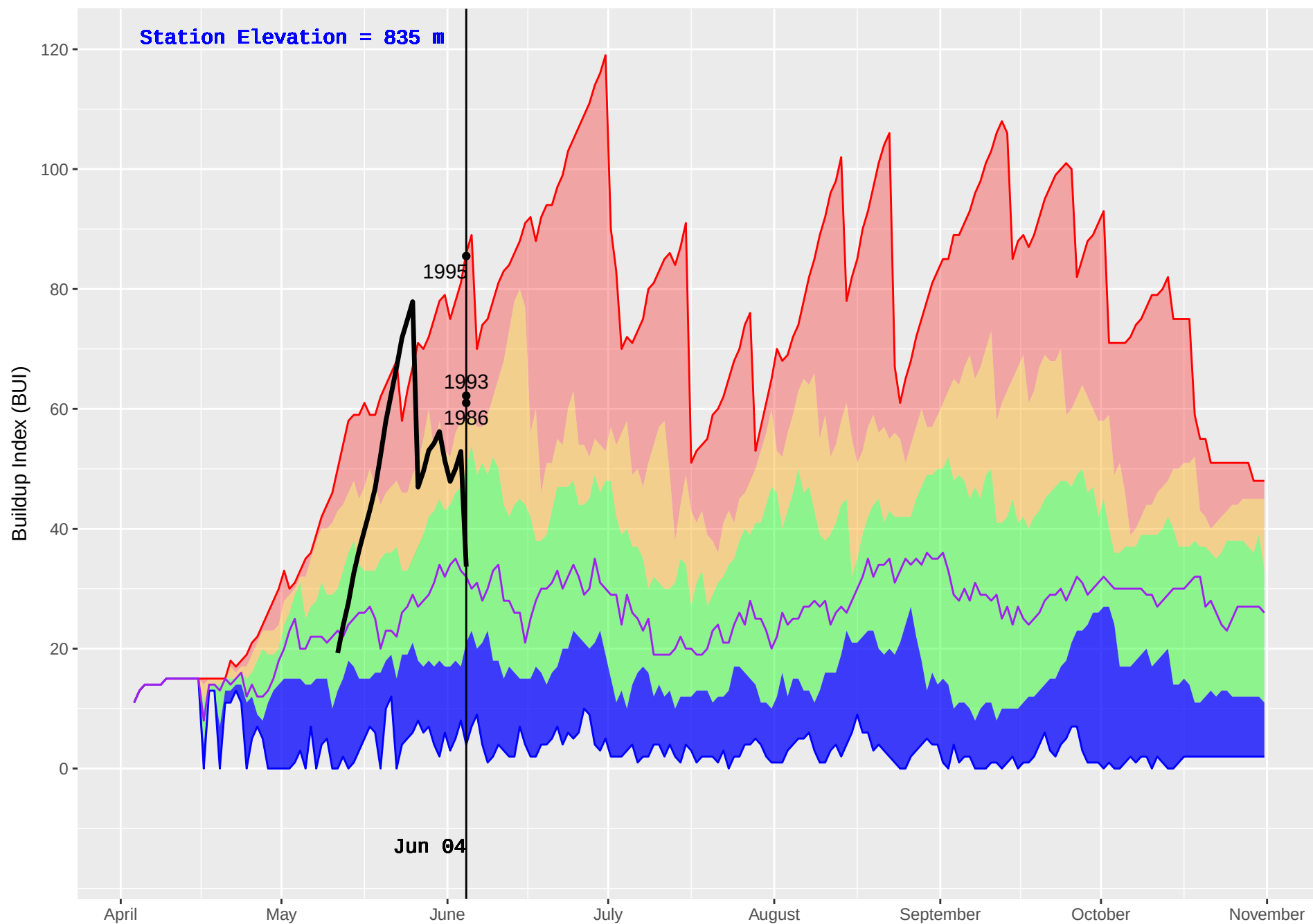
SILVER (120) : Historical (1986–2016) and Current (2018) Noon Buildup Index (BUI)
