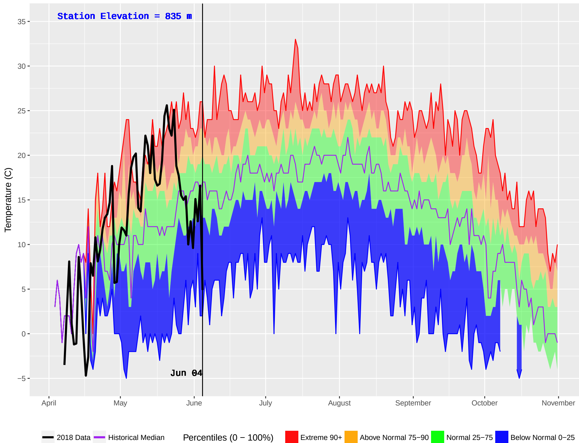
SILVER (120) : Historical (1986–2016) and Current (2018) Noon Temperature
